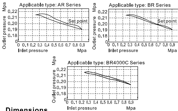
Pressure chart
